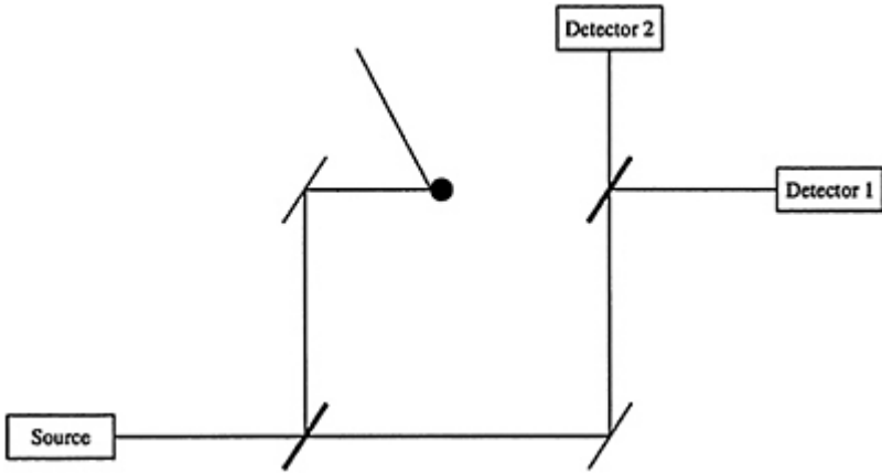
Figure A.2: Wave theory depicted in a Mach-Zehnder Interferometer with obstacle.
